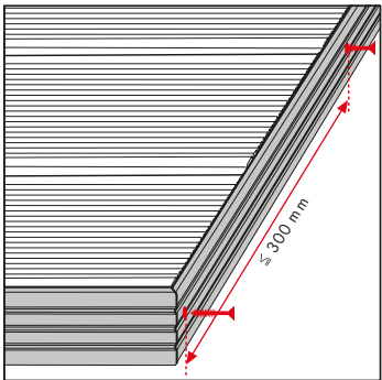
UPM PROFI DECK 150 RAIL STEP END CAP
