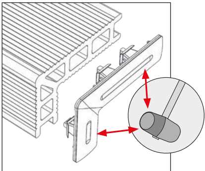
UPM PROFI DECK 150 RAIL STEP END CAP
